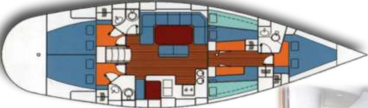
'ALPHA 51' layout - Skippeder yacht in Greece - Original pictures
